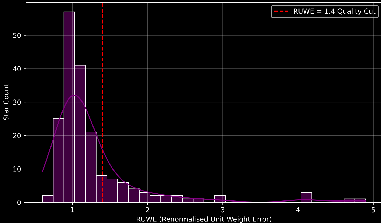
GAPOGEE DR17 Field [K2_C3_051-46] RUWE Distribution (n= 189)
