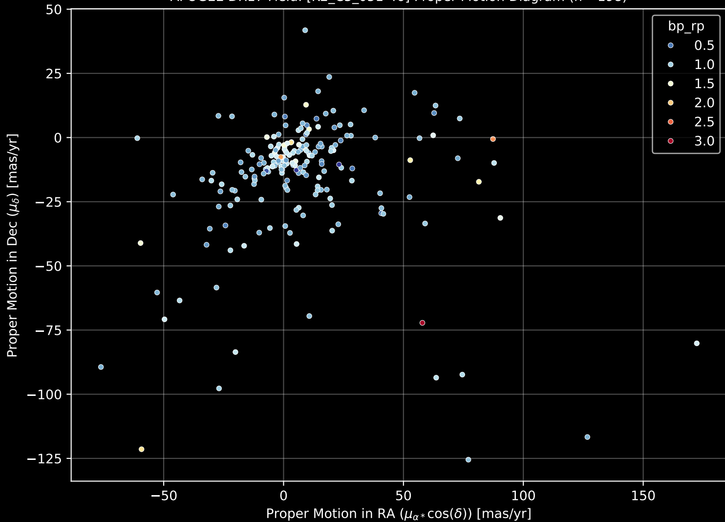
APOGEE DR17 Field: [K2_C3_051-46] Proper Motion Diagram (n= 198)
