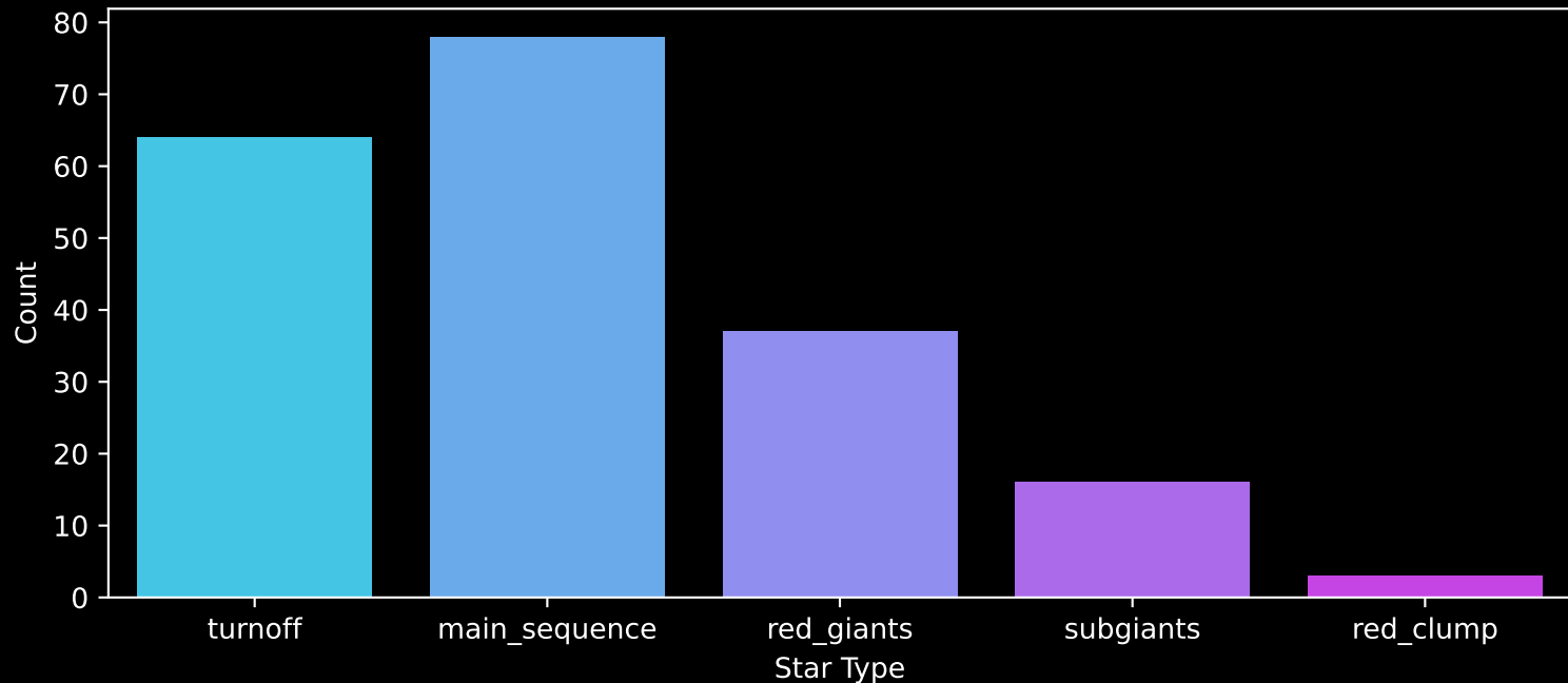
APOGEE DR17 Field: [K2_C3_051-46] Count plot of Star Type
