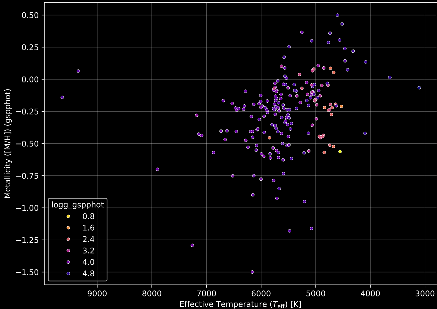
APOGEE DR17 Field: [K2_C3_051-46] Stellar Population Parameters (n= 198)
