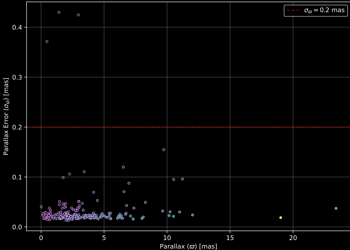
APOGEE DR17 Field: [K2_C3_051-46] Parallax Quality (n= 198)
